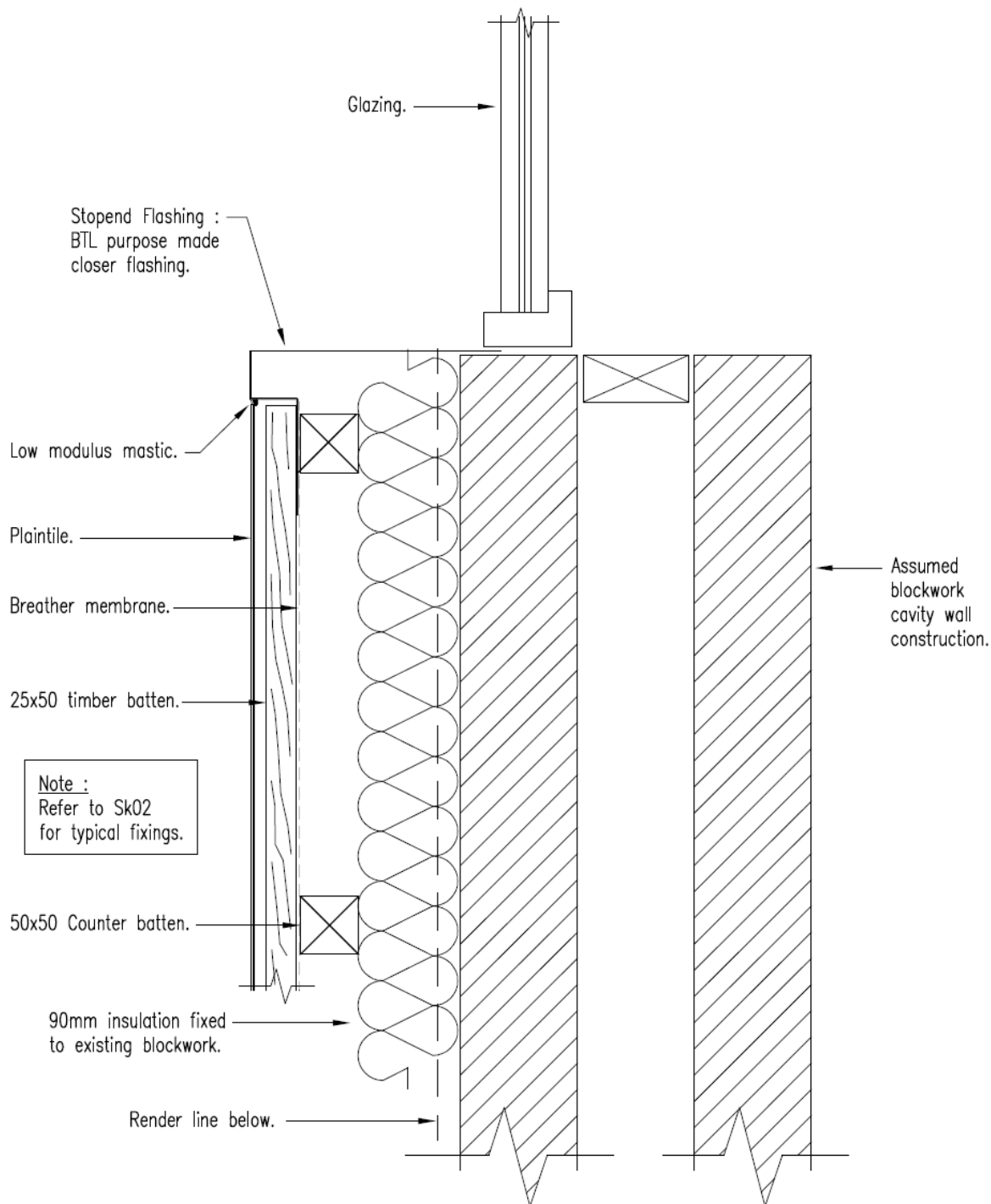
Plan View at Window Jamb.
